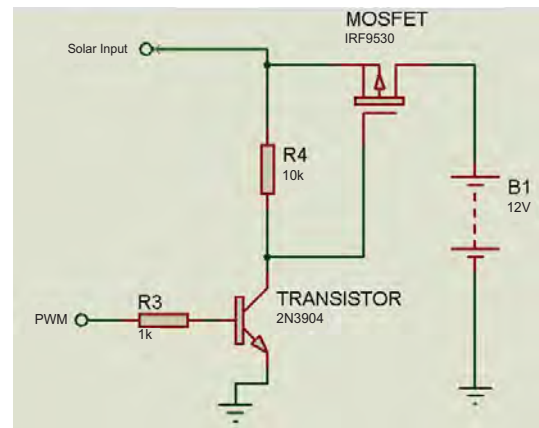
Fig. 5. Switching circuit for battery.
