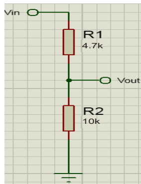
Fig. 4. Voltage divider for sampling.
