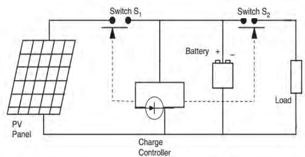
Fig. 1. System diagram of charge controller.
