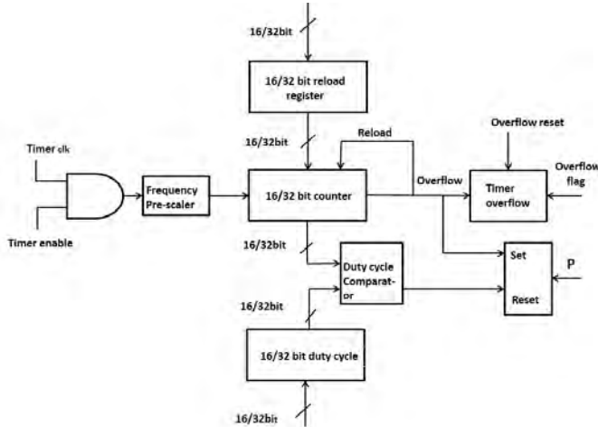
Fig. 9. PWM generation in TM4C123.
