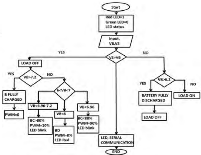
Fig. 10. Overall functional flow chart of the system.
