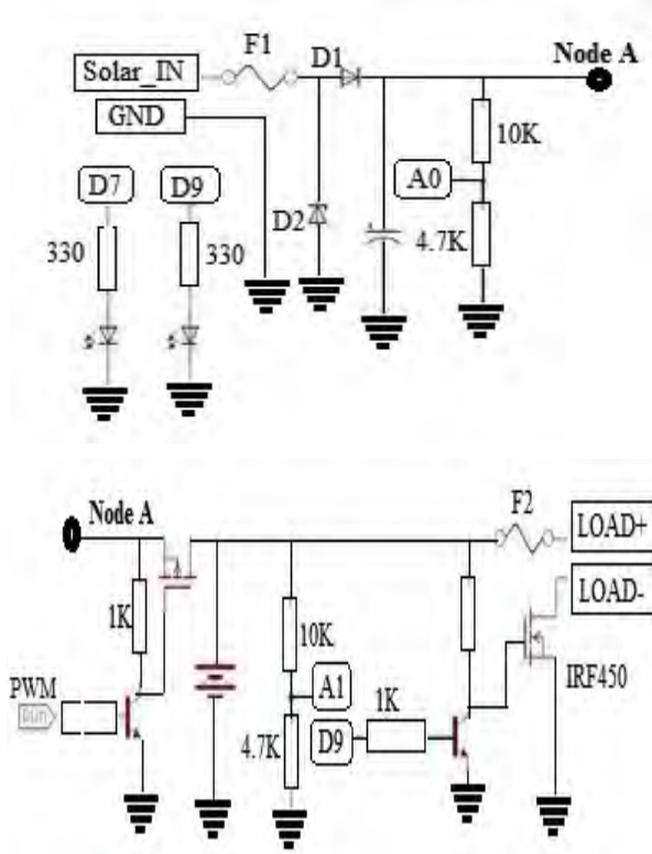
Fig. 6. Complete circuit of charge controller.
