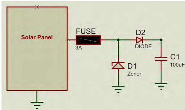
Fig. 3. Protection circuit for charge controller.
